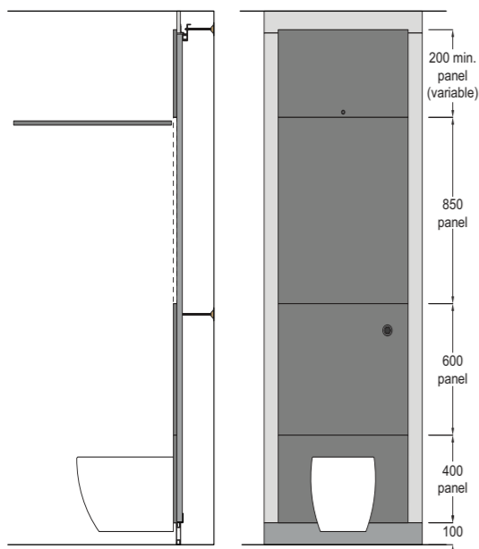
WC Hinged Panels
