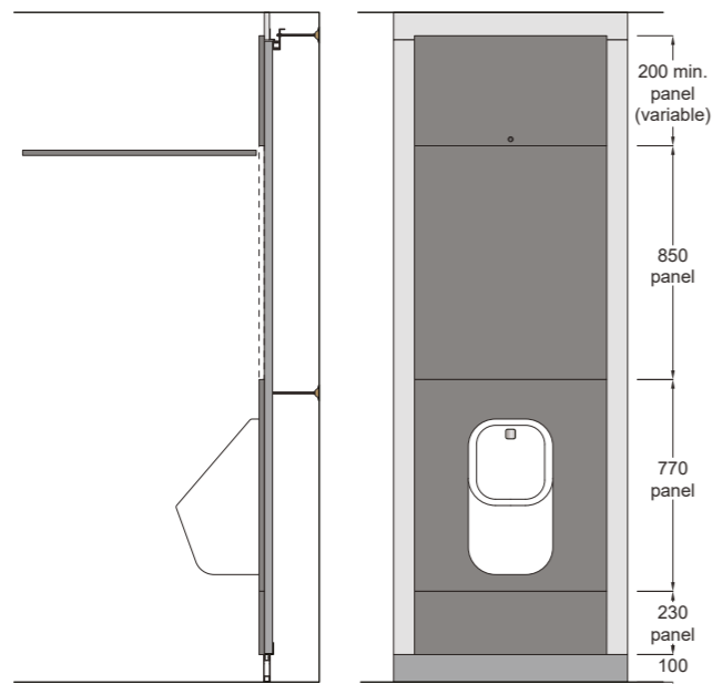
Urinal Hinged Panels
