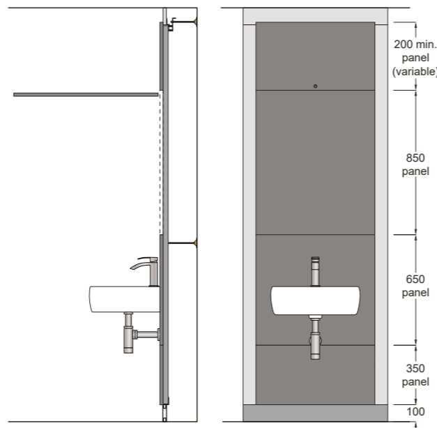
Washbasin Hinged Panels
