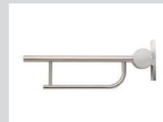
Hinged support rail Stainless steel Support rail in polished stainless steel with hinged support arm 800mm long and concealed fixing plate. L800 x H242 x W110mm Code: S6360MY
